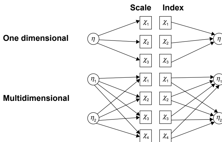
Figure 1 Types of multi-item questionnaires. Notes: \eta , \eta_k : Latent psychological variables; x_i : item scores.
