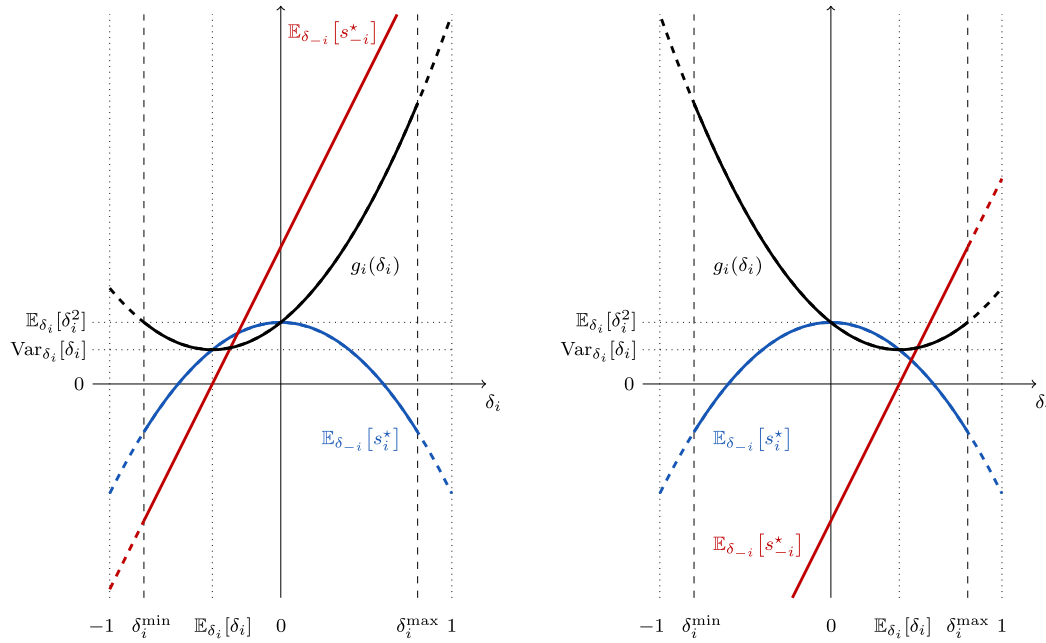
FIGURE 2. The utility gain g_i(\delta_i) = \mathbb{E}_{\delta_{-i}}[s_i(\delta)] + \delta_i \mathbb{E}_{\delta_{-i}}[s_{-i}(\delta)] > 0 that a social type \delta_i interim-expects under the transfer scheme s of (11), for two different type distributions, \delta_i \in [\delta_i^{\min}, \delta_i^{\max}] = [-4/5, 4/5] , \mathbb{E}_{\delta_i}[\delta_i] = \mp 2/5 , and \text{Var}_{\delta_i}[\delta_i] = 1/5 , such that \mathbb{E}_{\delta_{-i}}[s_i(\delta)] = 9/25 - \delta_i^2 , \mathbb{E}_{\delta_{-i}}[s_{-i}(\delta)] = 2\delta_i \pm 4/5 , and g_i(\delta_i) = (\delta_i \pm 2/5)^2 + 1/5 .
