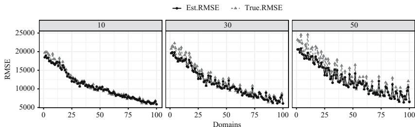
Fig. 1. RMSE of FH.MI estimator per domain for mean setting and varying nonresponse rates. Domains are ordered by increasing sample size.
