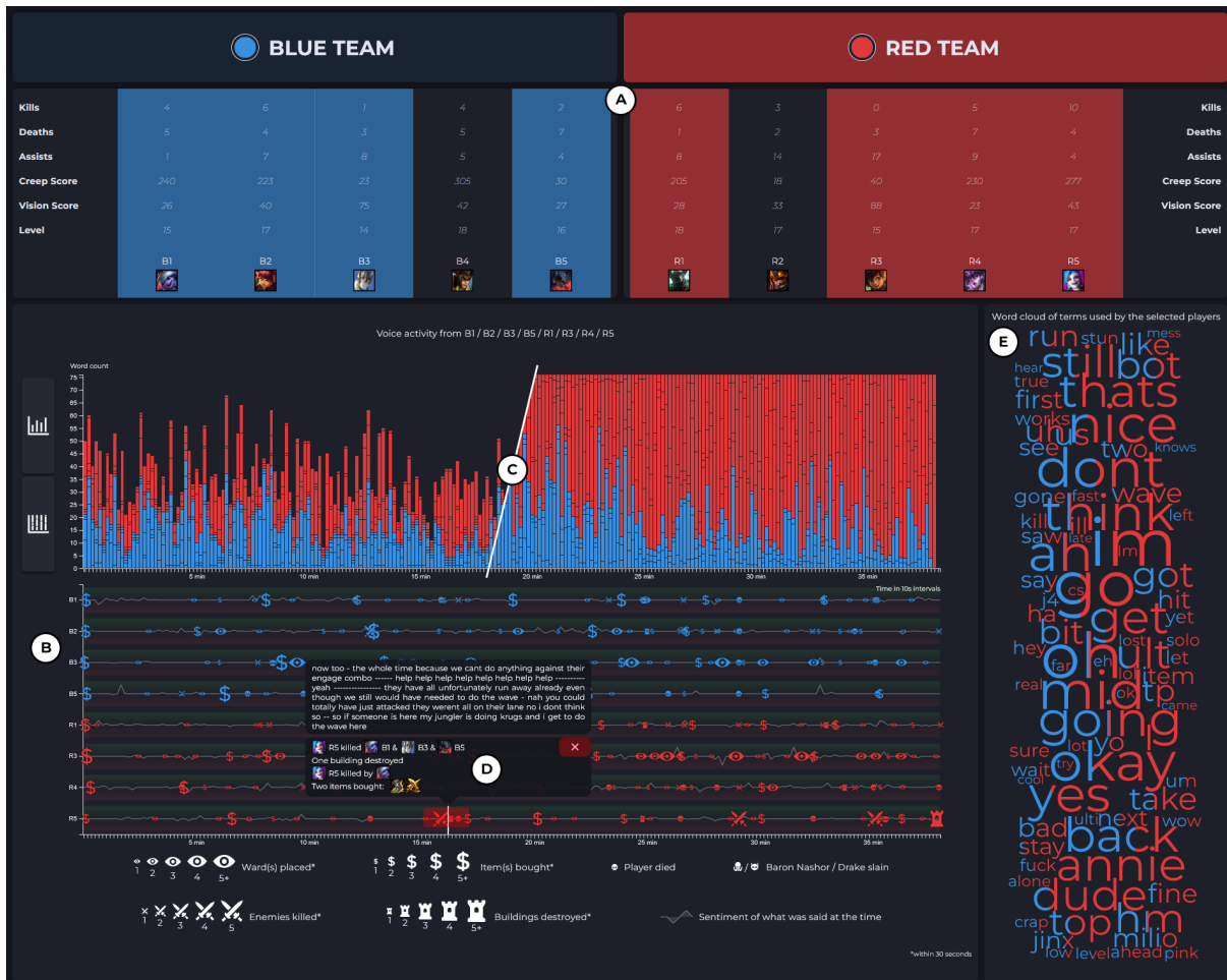
Figure 1: Overview of the visualization interface with scoreboard (A), timeline visualization (B) showing events and voice activity (C), details on the verbal communication (D), and enriched word cloud (E).
