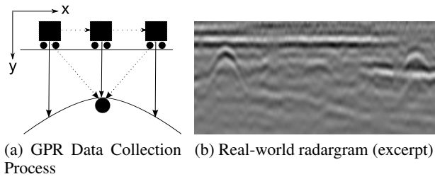
Figure 1: Hyperbolas are caused by steady movement of a radar vehicle across a buried pipe (a). At each horizontal position, an A-Scan (column) is measured, whose stacked visualization results in so-called radargrams, or B-Scans, (b).
