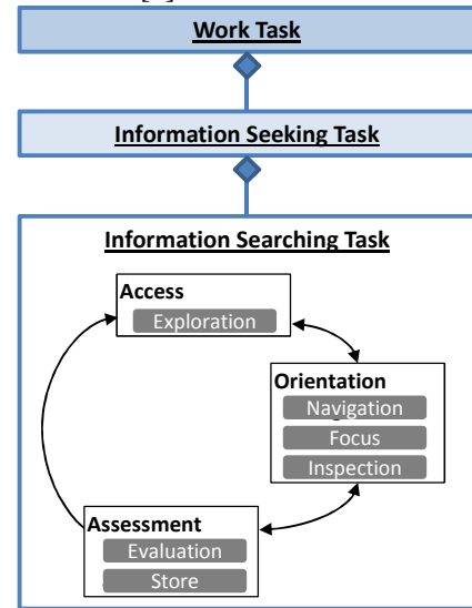
Figure 1: Task model of Byström and Hansen with integrated information searching activities as defined by Landwiche et al.
