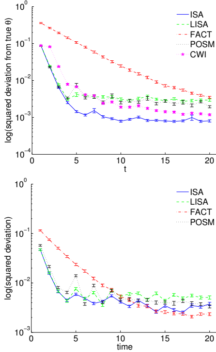
Figure 2: Squared deviations from true \theta for the constant (top) and the drift (bottom) setting.
