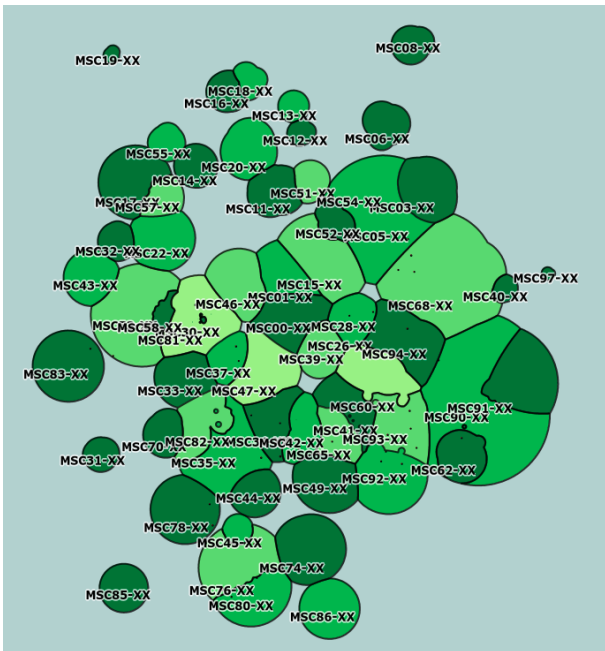
Figure 3: Geometry of the Math Subject Classifications
