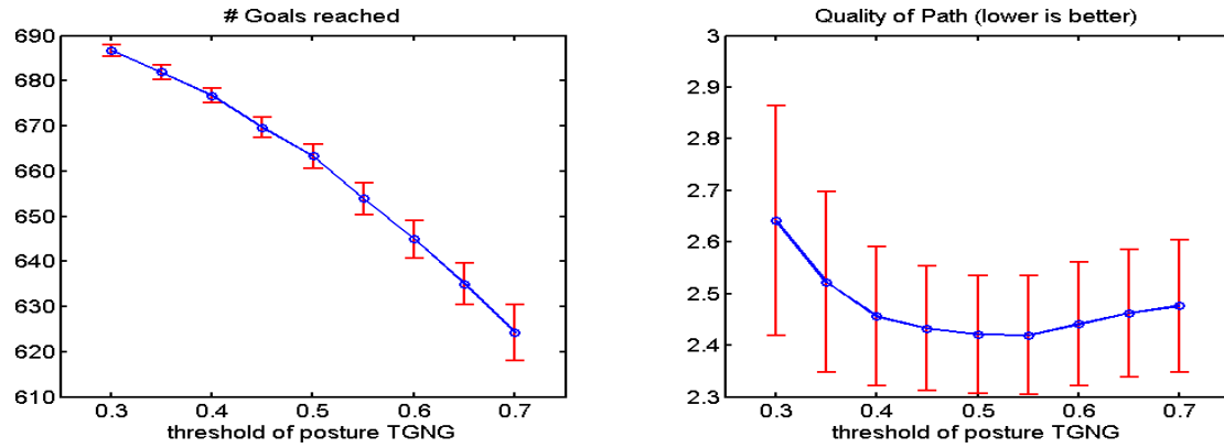
(c) Influence of posture space TGNG threshold parameter \theta_P .
