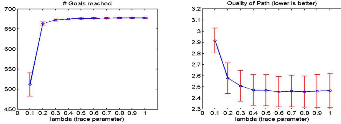
(b) Influence of activity trace parameter \lambda
