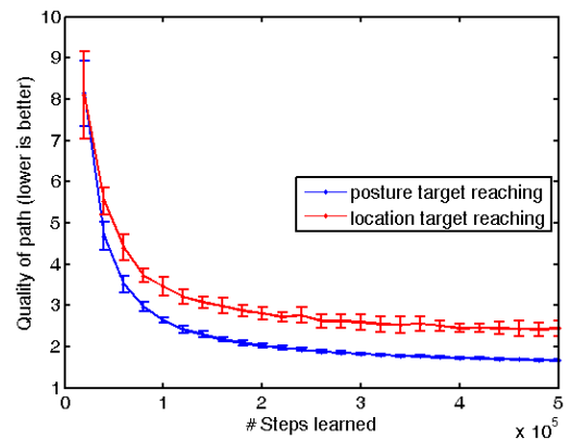
Figure 5: Also the path quality improves when a larger network is learned. Note that the system always attempts to move straight in posture space - thus the path quality for location goals has to be taken with a grain of salt. Nonetheless, there is definite room for improvement when considering the path quality results.
