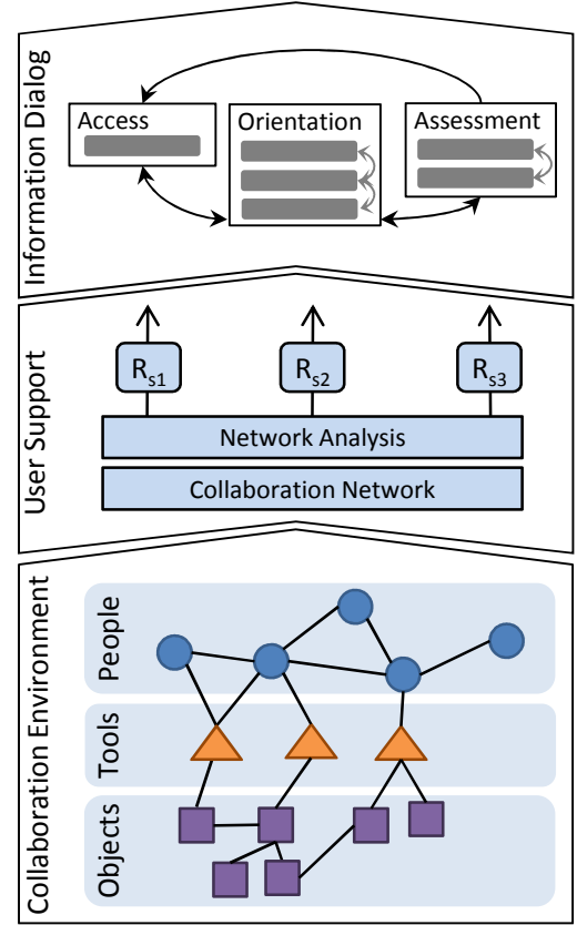
Figure 8: Layer model for supporting a group during IS&S tasks
