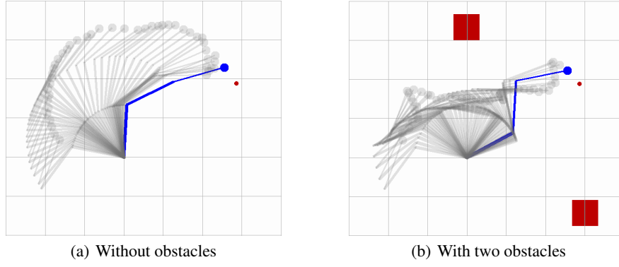
Figure 3: Two reaching movements, (a) without obstacles and (b) with two obstacles (red squares). The arm has to move its end effector to the location goal target (small red circle). The trajectory taken by the arm is visualized in light gray color. The resulting posture when the target was (nearly) reached is shown in blue. Due to the obstacles in (b) the resulting trajectory differs, effectively avoiding crashing into the upper obstacle.
