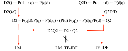
Figure 1: The D2Q2 framework.
