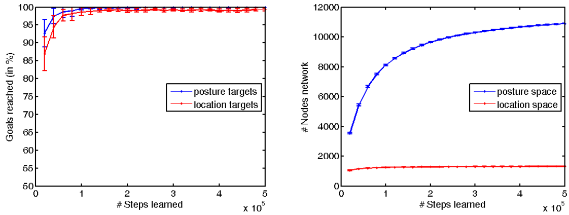
Figure 4: With even lower TGNG thresholds, the networks grow bigger and the target reaching performance also reaches close-to 100% even when reaching for location targets.
