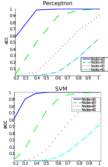
Figure 2: Performance on artificial data for perceptrons (top) and SVMs (bottom).
