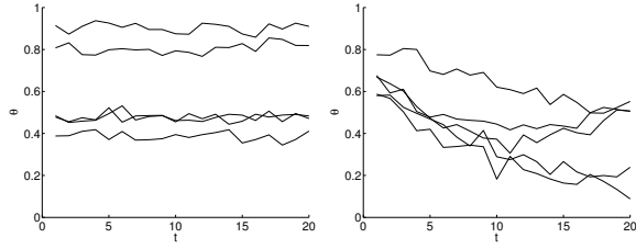
Figure 1: Randomly parametrized functions modelling \theta in absence (left) and presence of drift (right). In both scenarios white noise is added.
