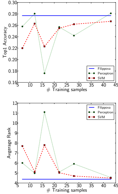
Figure 3: Results on news headlines: Accuracies and average ranks for perceptrons and SVMs.
