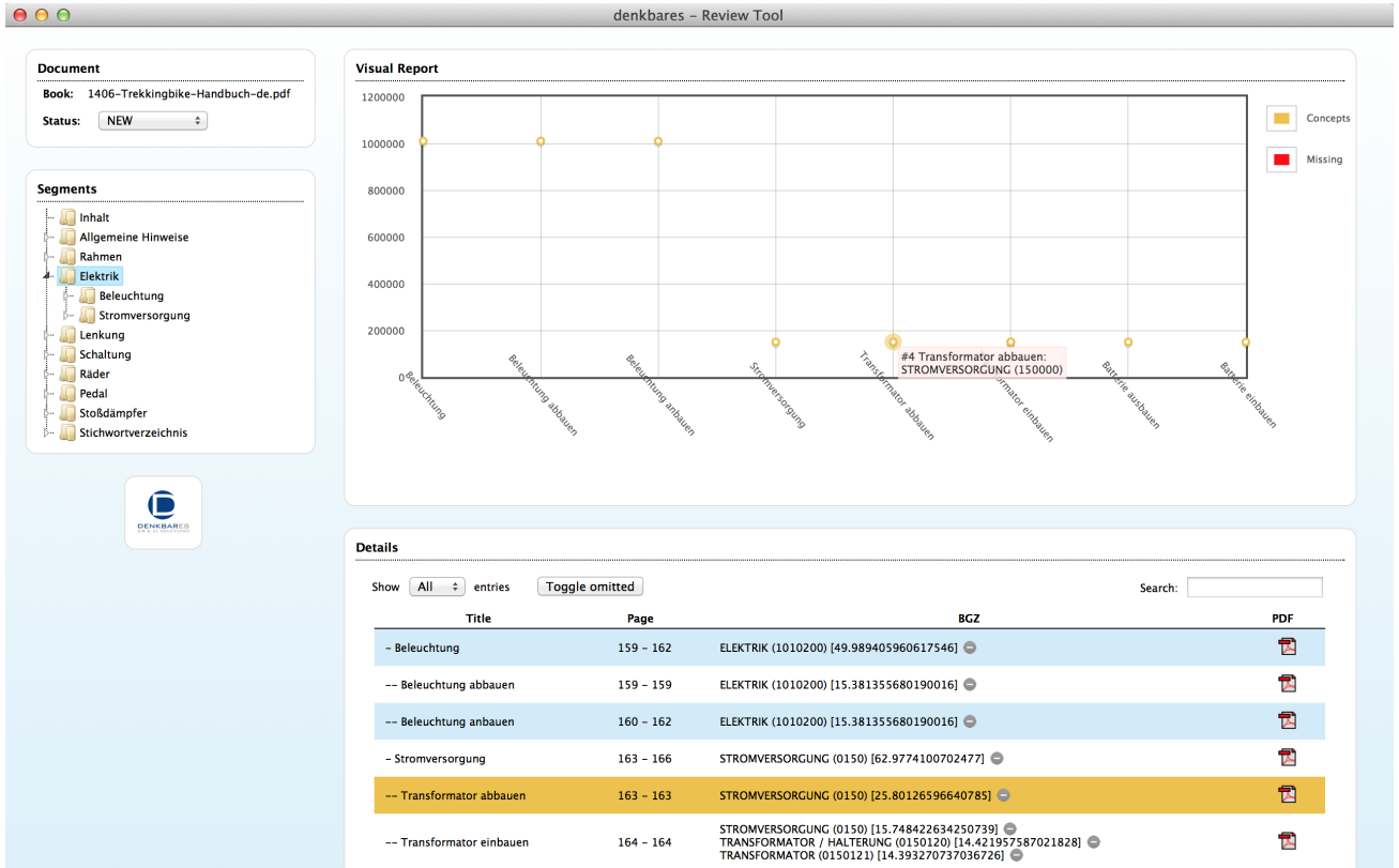
Figure 4: A tool for the manual review of semantic annotations, containing the hierarchical segmentation (left), a visual report (top right) and a detail view (bottom right).
