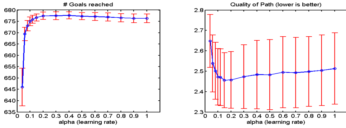
(a) Influence of learning rate parameter \alpha .
