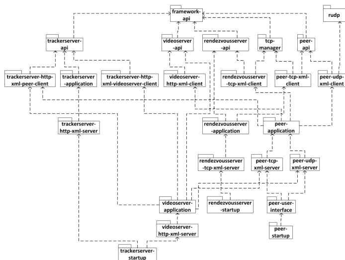
Figure 2. UML Packet Diagram of the Framework
