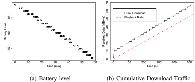
Figure 7. Test Run Results (continued)
