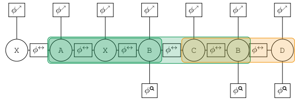
Figure 1: A linear-chain CRF can only model probabilities of labels occurring at particular positions ( \phi^l ), and probabilities for labels being adjacent to one another ( \phi^{l,l+1} ). In particular, linear-chain CRFs cannot encourage or discourage the presence of nonlocal patterns in the label sequence, e.g. the regular expression patterns A.*B and C.*D . With an RPCRF, a set of such patterns can be specified, and the model can learn the probability of each of those patterns occurring at different positions of the label sequence ( \phi^a ).
