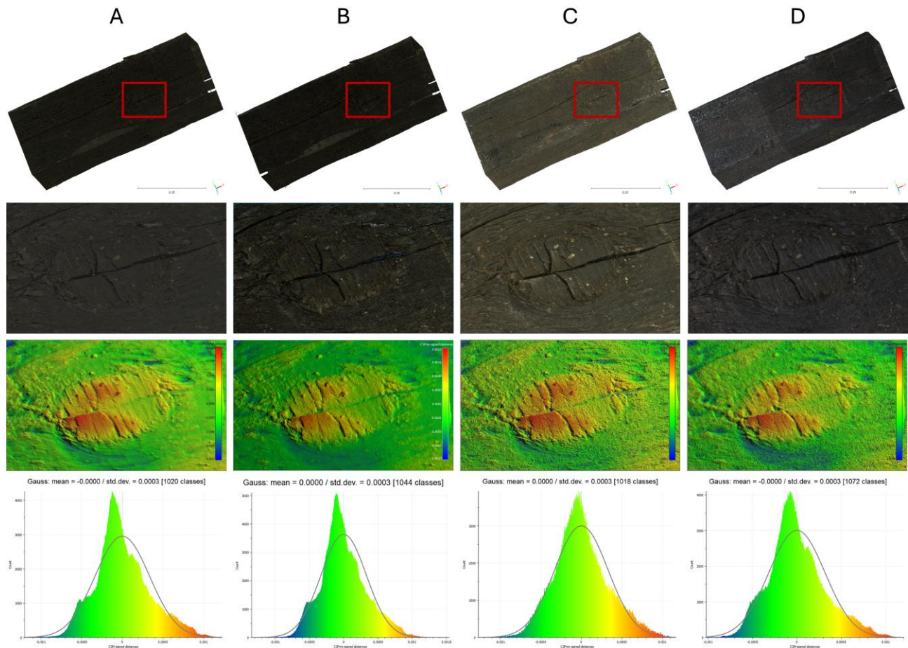
Figure 7: Comparison of the 3D models of the four datasets: point clouds couled by RGB full (top), detailed pointcloud of a knot coloured in RGB and by height (second and third row) and histograms for the heigth differences to the best-fit plane (bottom).
