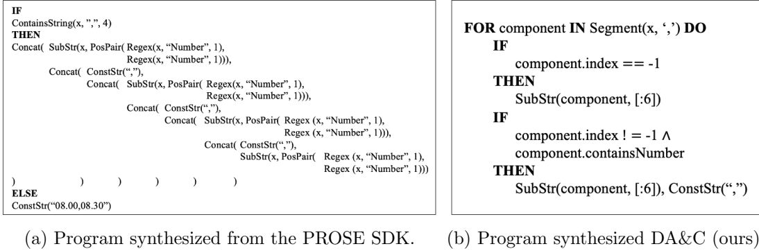
Figure 2: A divide, align, & conquer (DA&C) strategy yields a compact and well-generalizing program for the task in Figure 1b.
