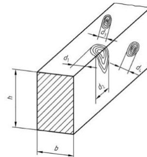
Figure 1. The determination of the largest single branch by the dimension of knot (DIN, 2003).
