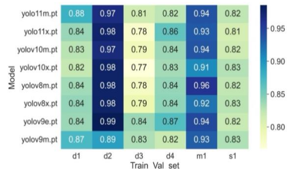
Figure 5. F1-score heatmap from from validation results: Each cell shows the F1-score of a particular model Y (rows) trained and validated on the dataset X (columns). These scores were recorded during training and reflect model performance on their respective validation sets.
