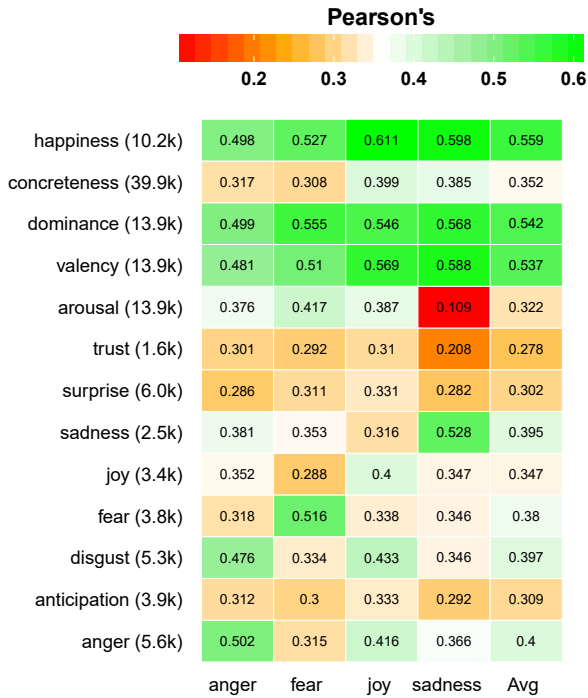
Figure 2: Pearson’s correlation of single rating categories (Y-Axis) on each target emotion (X-Axis). Numbers in brackets refer to training size used to extend the norms. Evaluation based on 10-fold cross validation using the full training data and random forest.
