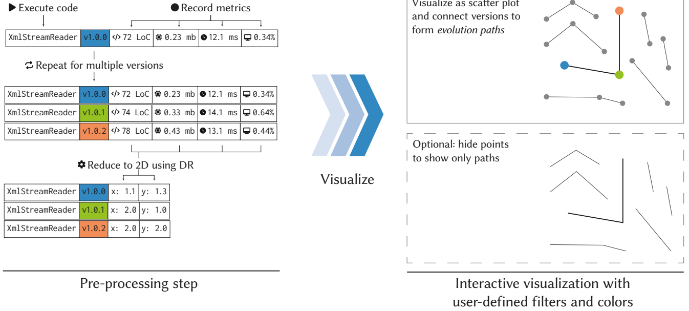
Figure 1: We consider the evolution of high-dimensional performance data of software artifacts and reduce the multidimensional vectors containing the recorded metrics down to two dimensions. In the resulting scatter plot, we connect adjacent software versions to form temporal trajectories, that we call evolution paths .
