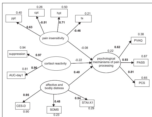
Figure 2 ) Structural equation model prediction of psychological mechanisms of pain processing by the factors ‘affective and bodily distress’, ‘pain insensitivity’ and ‘cortisol reactivity’. Standardized beta coefficients (presented next to each pathway) and values of R 2 (presented next to each indicator variable and predicted variable) are reported. Significant results are marked in bold. AUC Area under the cortisol at the time of awakening response curve; CES-D Center for Epidemiologic Studies Depression Scale; cpt Cold pain threshold; hpt Heat pain threshold; PASS Pain Anxiety Symptoms Scale; PCS Pain Catastrophizing Scale; ppt Pressure pain threshold; PVAQ Pain Vigilance and Awareness Questionnaire; SOMS Screening for Somatoform Symptoms; STAI-X1 State-Trait Anxiety Inventory (State Anxiety); ts Temporal summation of heat pain
