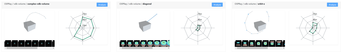
Figure 2: One row in the Dataset Explorer (Section 4.1) showing for each camera path an interactive 3D abstraction of the path, rendered sample images, and aggregated performance metrics. Depicted are three of the nine recorded paths of the OSPRay example (Section 5.1).
